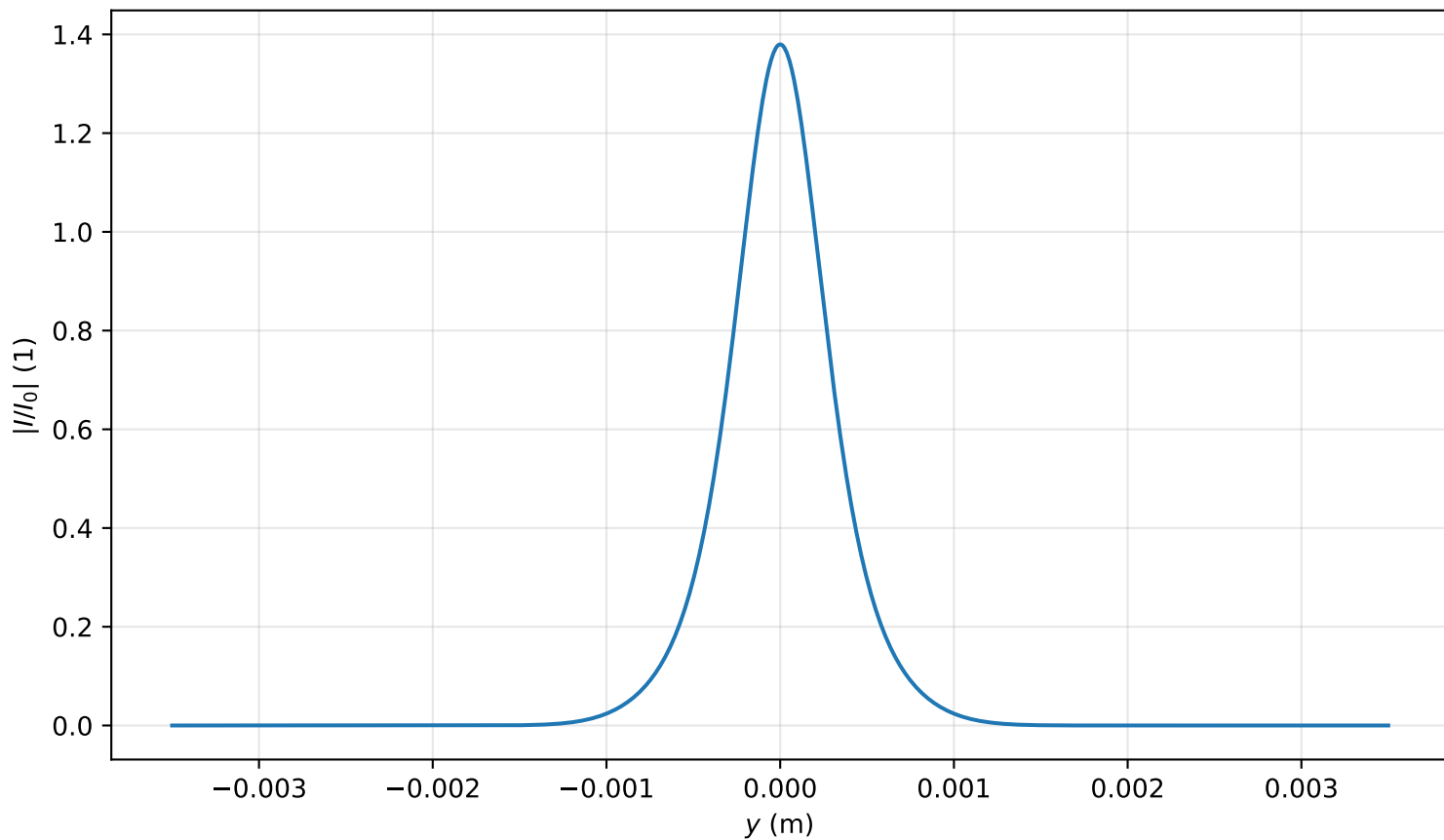
Intensity profile I(x=0, y, z=0.955)/I_0 , P_{in}=0.9P_{cr} , artificial time
